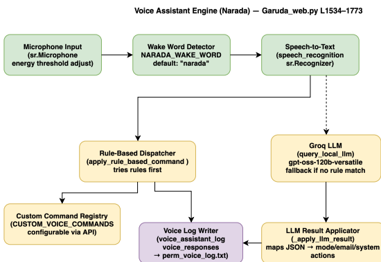
FIGURE 8. Voice assistant Narada. Microphone capture, wake-word gate, speech-to-text, rule-based dispatcher, and Groq LLM fallback for open-ended intents.
