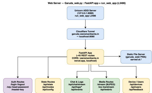
FIGURE 11. Web server. FastAPI under Uvicorn behind a Cloudflare tunnel, with ~45 REST routes and three parallel media channels (MJPEG, WebSocket, WebRTC).
